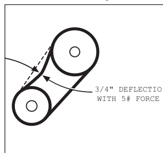
Figure 14.3 - Belt Tension Adjustment
