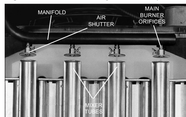
Figure 16.3 - Air Shutter Adjustment, Propane Gas
