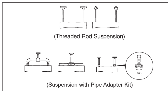
Figure 5.2 - Suspension Methods
