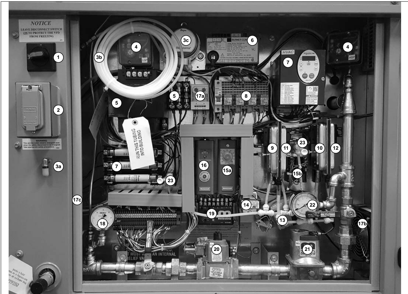
Figure 8.1 - Standard Feature and Factory Mounted Option Locations - Control Cabinet
