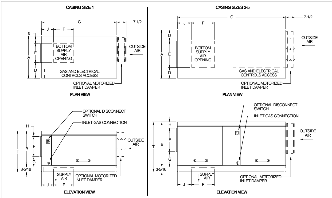
Figure 18.1 - Unit Dimensions (without Evap Cooler or Side Access Filter Section) (inches)
