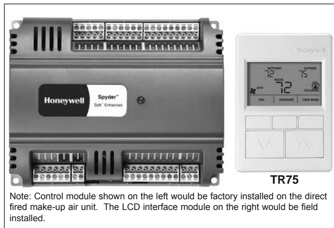
Figure 15.1 - Honeywell SPYDER Controller/Interface
