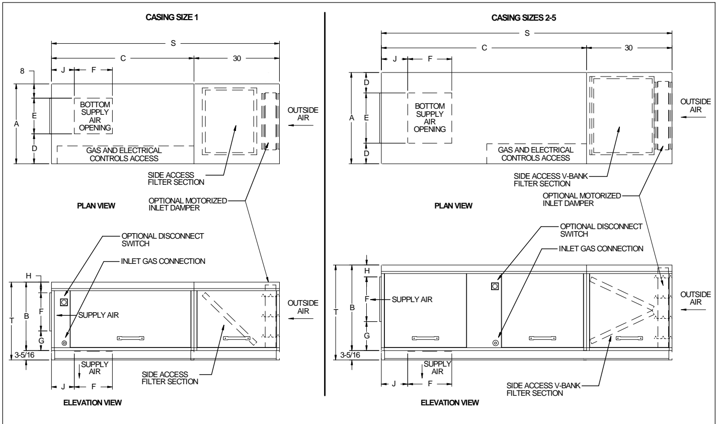
Figure 19.1 - Unit Dimensions (with Side Access Filter Section) (inches)
